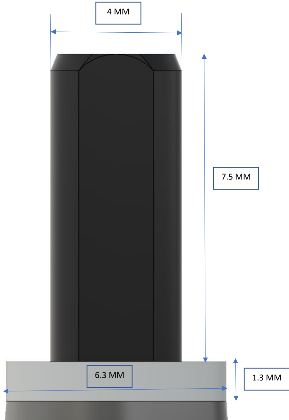
Tuner Front View
