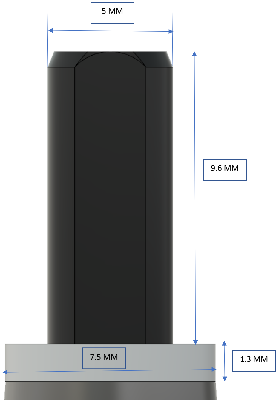
Tuner Front View (Bass)
