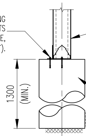
TYPICAL PILE DETAIL SCALE: 1:20
