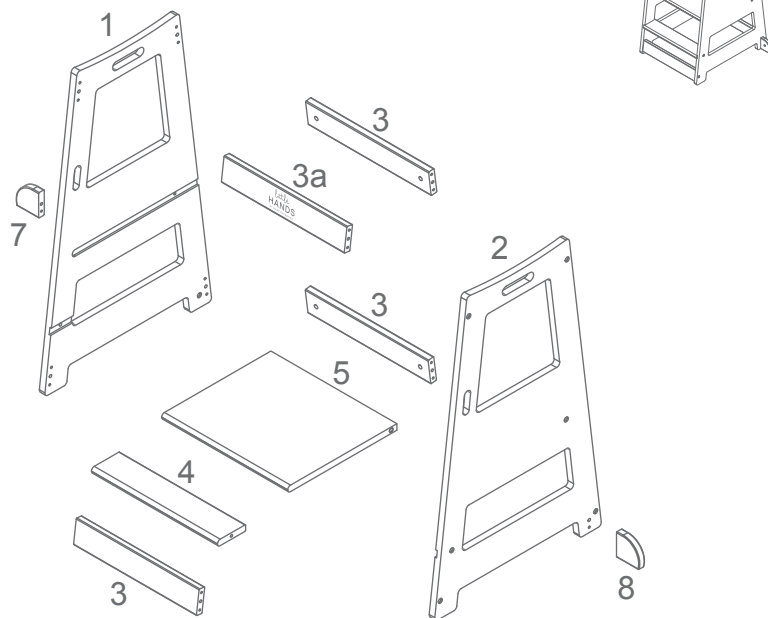
5. Foot Panel
