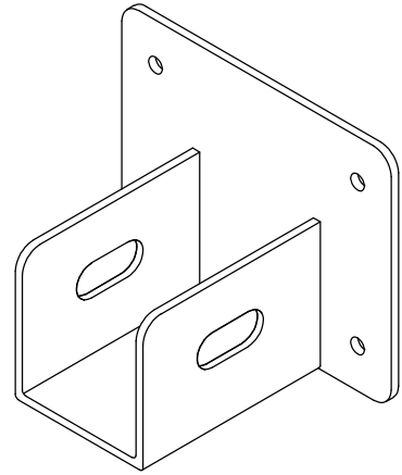
HW20674 (45*76*25mm)
