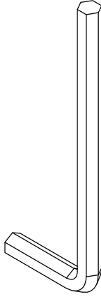
HW20615 (57*30*4mm)
